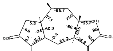
Fig. 2. Torsion angles ( ^\circ ). E.s.d.'s are in the range 0.3–0.6 ^\circ .
