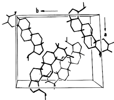
Fig. 2. The unit-cell contents viewed down the c axis.
