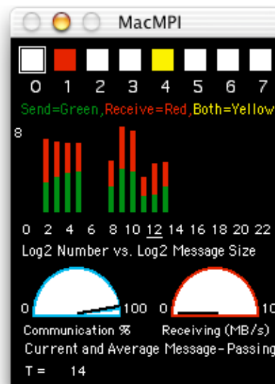
Figure 3. The monitor window of MacMPI, which keeps track of statistics about the execution of the running parallel application.
